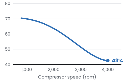
Volumetric efficiency
