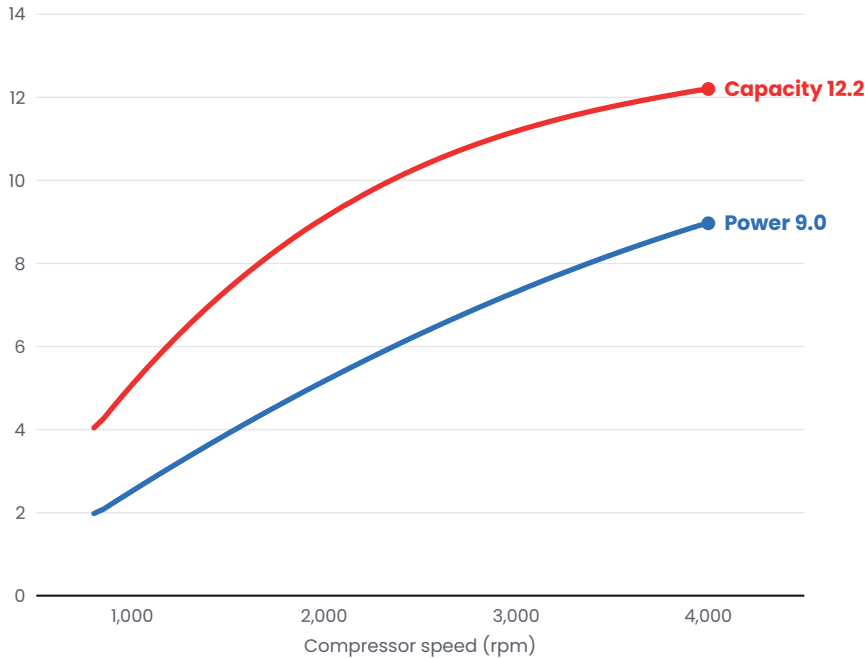
Capacity and power input
